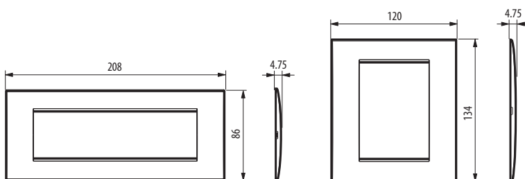
LNC4807...
