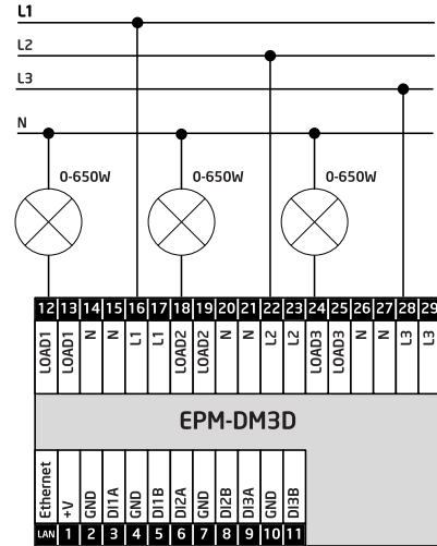
Three phases. Three loads.
