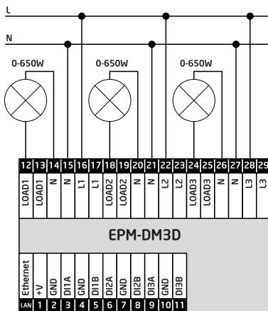
One phase. Three loads. Using "N" terminal for connection
