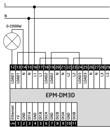
One phase. One load. Three channels are combined.
