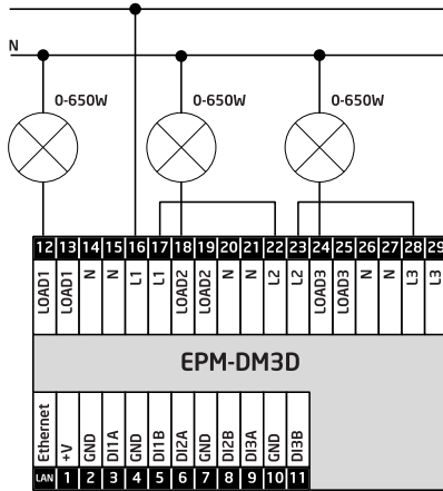
One phase. Three loads.
